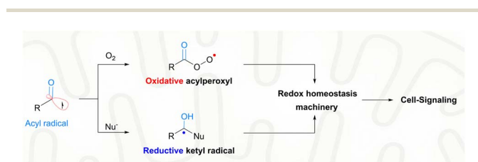
Fig. 1 The chemical reactivities of acyl radicals to fine-tune the cellular redox homeostasis.
