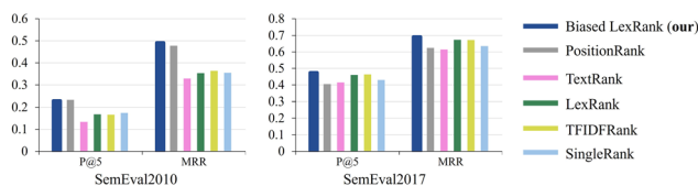
Fig. 10 The result of the proposed biased LexRank is compared with the baseline using various metrics on SemEval2010 and SemEval2017.
