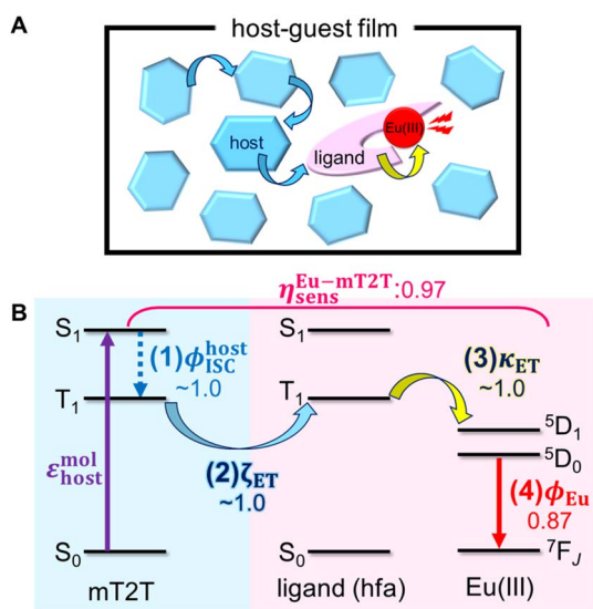
Fig. 6 Overview of inter- and intra-molecular energy transfer processes in the Eu-mT2T film. (A) Schematic in real space. (B) Schematic of energy levels. \phi_{\text{ISC}}^{\text{host}} , \zeta_{\text{ET}} , \kappa_{\text{ET}} , and \phi_{\text{Eu}} represent the quantum yields of (1) ISC in mT2T, (2) inter-molecular energy transfer from mT2T to the hfa ligands, (3) intra-molecular energy transfer from the hfa ligands to the Eu(III) ion, and (4) the emission in the Eu(III) ion, respectively. \eta_{\text{sens}}^{\text{Eu-mT2T}} is the overall photosensitization efficiency in the Eu-mT2T film (eqn (4)).
