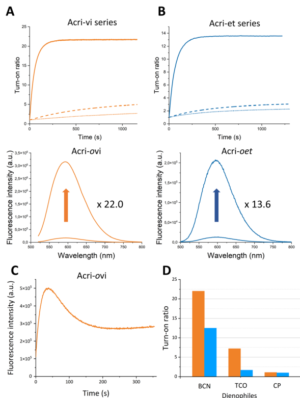
Fig. 2 Fluorescence enhancement of (A) Acri-vi and (B) Acri-et fluorogenic dyes (2 \mu M) upon the addition of BCN (20 \mu M) in 10 mM sodium cacodylate buffer (100 mM NaCl and pH 7.4) containing BSA (200 \mu M). Ortho , meta and para derivatives are represented by solid, dashed and dotted lines, respectively. (C) Fluorescence enhancement of (C) Acri-ovi (0.5 \mu M) upon the addition of TCO (50 \mu M) and of (D) fluorogenic dyes Acri-ovi (in orange) and Acri-oet (in blue) (2 \mu M) upon the addition of BCN, TCO or CP (20 \mu M), in 10 mM sodium cacodylate buffer (100 mM NaCl and pH 7.4) containing BSA (200 \mu M).
