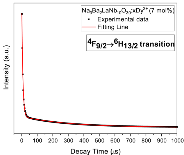
Fig. 18 Decay curve 4F_{9/2} \rightarrow 6H_{13/2} transition in \text{Na}_3\text{Ba}_2\text{LaNb}_{10}\text{O}_{30}:\text{xDy}^{3+} ( x = 7 mol%) phosphor.
