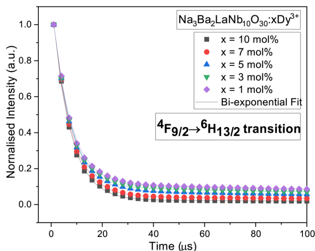
Fig. 19 Decay curves for 4F_{9/2} \rightarrow 6H_{13/2} transition in \text{Na}_3\text{Ba}_2\text{LaNb}_{10}\text{O}_{30}:\text{xDy}^{3+} ( x = 1, 3, 5, 7 and 10 mol%) phosphors.
