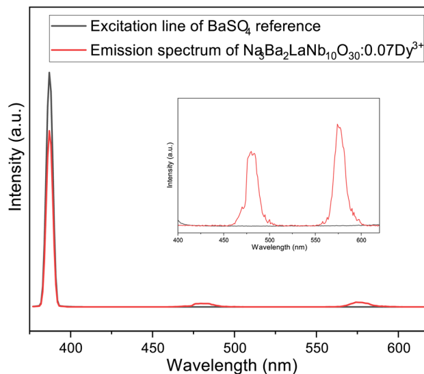
Fig. 20 Excitation and emission spectra of \text{Na}_3\text{Ba}_2\text{LaNb}_{10}\text{O}_{30}:\text{xDy}^{3+} ( x = 7 mol%) phosphor and \text{BaSO}_4 reference using an integrating sphere for IQE measurement. Inset: enlarged emission spectra (400–630 nm).
