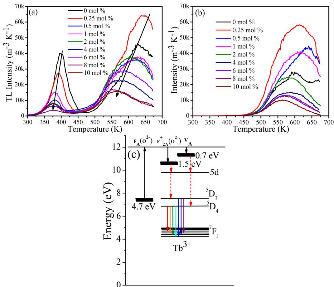
Fig. 8 TL glow curve of CaF 2 :Tb 3+ after 5 min of (a) UV (254 nm) and (b) blue (486 nm) irradiation. (c) Schematic energy level diagram for defects and Tb 3+ ions.
