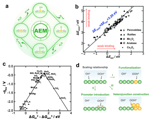
Fig. 3 (a) Schematic illustration of the AEM. (b) The function of the adsorption energies ( \Delta E ) of HOO* with HO* on various catalysts. (c) The volcano plot for the theoretical overpotential as a function of the adsorption-free energy difference between O* and HO*. (b and c) Reproduced with permission from ref. 40. Copyright 2011, Wiley-VCH. (d) Schematic of strategies for breaking the scaling relationship in OER.
