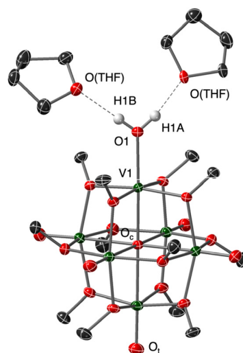
Fig. 3 Molecular structure of [\text{V}_6\text{O}_6(\text{OH}_2)]^{0-} shown with 50% probability ellipsoids. Selected hydrogen atoms have been omitted for clarity. Key: dark green ellipsoids: V; red ellipsoids: O; dark grey ellipsoids: C; white spheres: H.
