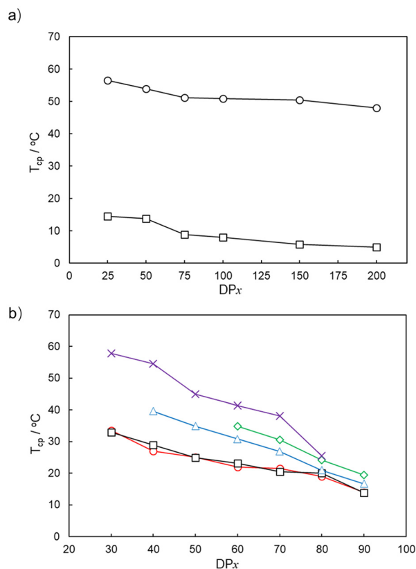
Fig. 5 Dependence of the cloud-point temperature ( T_{cp} ) on the degree of polymerization ( DP_x ) of (a) (□) PEOAm x and (○) PMOEAm x and (b) (○) PDAm y -b-PEOEAm x , (□) PEOAm x -b-PDAm y , (◇) PDAm y -b-PEOEAm x -b-PDAm y , (Δ) PEOAm x -b-PDAm y -b-PEOEAm x , and (×) (PDAm y/2 -b-PEOEAm x/2 ) 2 .
