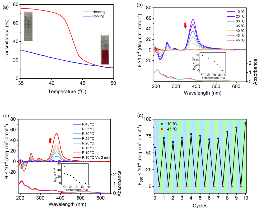
Fig. 7 Plots of transmittance versus temperature for the aqueous solution ( C = 1.0 \text{ mg mL}^{-1} ) of SP-GA-MeG1 at a heating rate of 0.5 \text{ °C min}^{-1} (a). CD and UV/vis spectra of aqueous solutions ( 0.3 \text{ mg mL}^{-1} ) of SP-GA-MeG1 with the temperature increased from 10 to 45 °C (b) and decreased from 45 to 10 °C (c), and the first Cotton effect at 380 nm ( \theta_{380} ) after several cycles of heating and cooling through irradiation with visible light (d). Heating or cooling rate = 2.0 \text{ °C min}^{-1} ; \lambda_{\text{vis}} > 450 \text{ nm} . The inset in (a): photographs of the aqueous solutions below and above the T_{\text{cp}} . Insets in (b) and (c): plots of molar ellipticity ( \theta_{380} ) against temperature.
