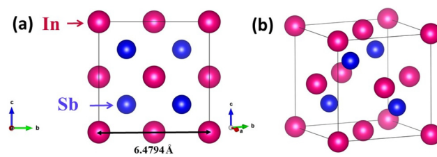
Fig. 1 (a) Top view of bulk InSb and (b) atomic structure of bulk InSb.
