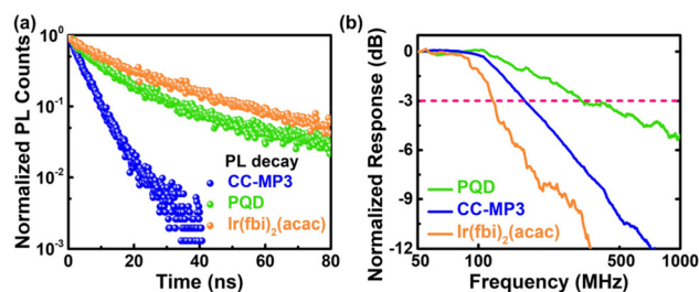
Fig. 6 (a) PL decay curve of neat CC-MP3, neat PQDs, and neat Ir(fbi) 2 (acac) films. (b) -3 dB bandwidth of emitters.
