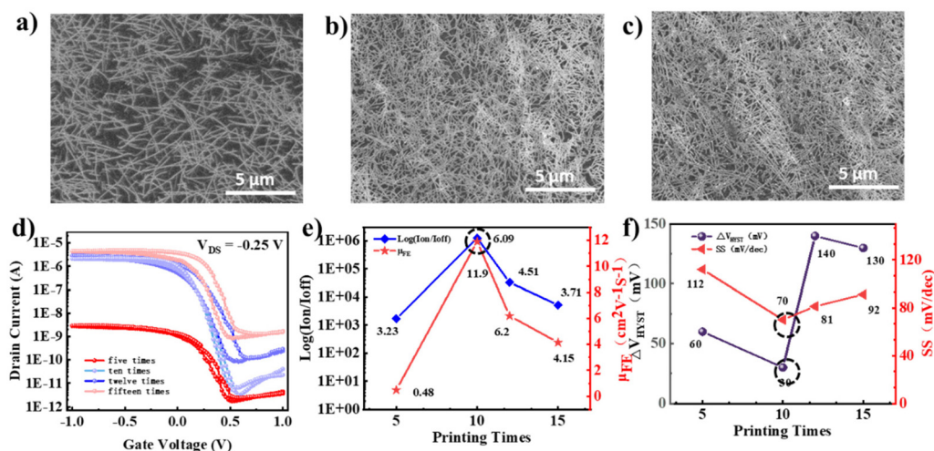
Fig. 4 SEM images of R2R gravure printed SWCNT thin films with different printing times using sc-SWCNT inks with the adsorption peak height of 1.8. (a) 5 times, (b) 12 times, and (c) 15 times, (d) the corresponding transfer curves, (e) calculated I_{on}/I_{off} and \mu_{FE} , and (f) SS and \Delta V_{HYST} of fully printed SWCNT-TFTs.
