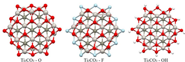
Fig. 9 Optimized structures of the studied \text{Ti}_2\text{CO}_2\text{-X} QDs with different edge functionalization ( X = \text{O}, \text{F}, \text{OH} ). Titanium, carbon, oxygen, fluorine, and hydrogen atoms are shown in light grey, dark grey, red, light blue, and white, respectively.
