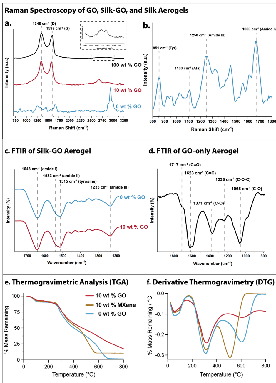
Fig. 5 (a) Raman spectra for 100 wt% GO ( 4 \text{ mg mL}^{-1} GO); silk aerogels (10, 0 wt% GO). (b) Raman spectra highlighting 800–1800 \text{cm}^{-1} for silk-only aerogels (0 wt% GO). (c) FTIR of silk aerogels (0, 10 wt% GO). (d) FTIR of 100 wt% GO aerogel ( 4 \text{ mg mL}^{-1} GO). (e) Thermogravimetric analysis (TGA) and (f) derivative thermogravimetry (DTG) of pulverized silk aerogels (10, 0 wt% GO and 10 wt% MXene).
