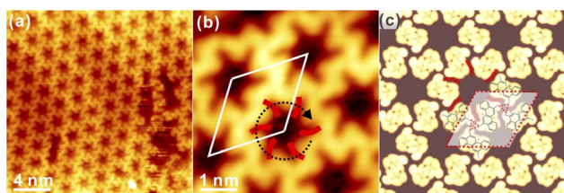
Fig. 2 (a) Increasing coverage to 1 ML leading to the linkage of hexagonal structure into 2D network in a large area, and (b) the high-resolution STM with the unit cell indicated. (c) The optimized configuration by DFT overlaid on top of the simulated STM image. U_{\text{bias}} = -1.3 V for (a) and 1.3 V for (b); I_t = 0.1 nA.
