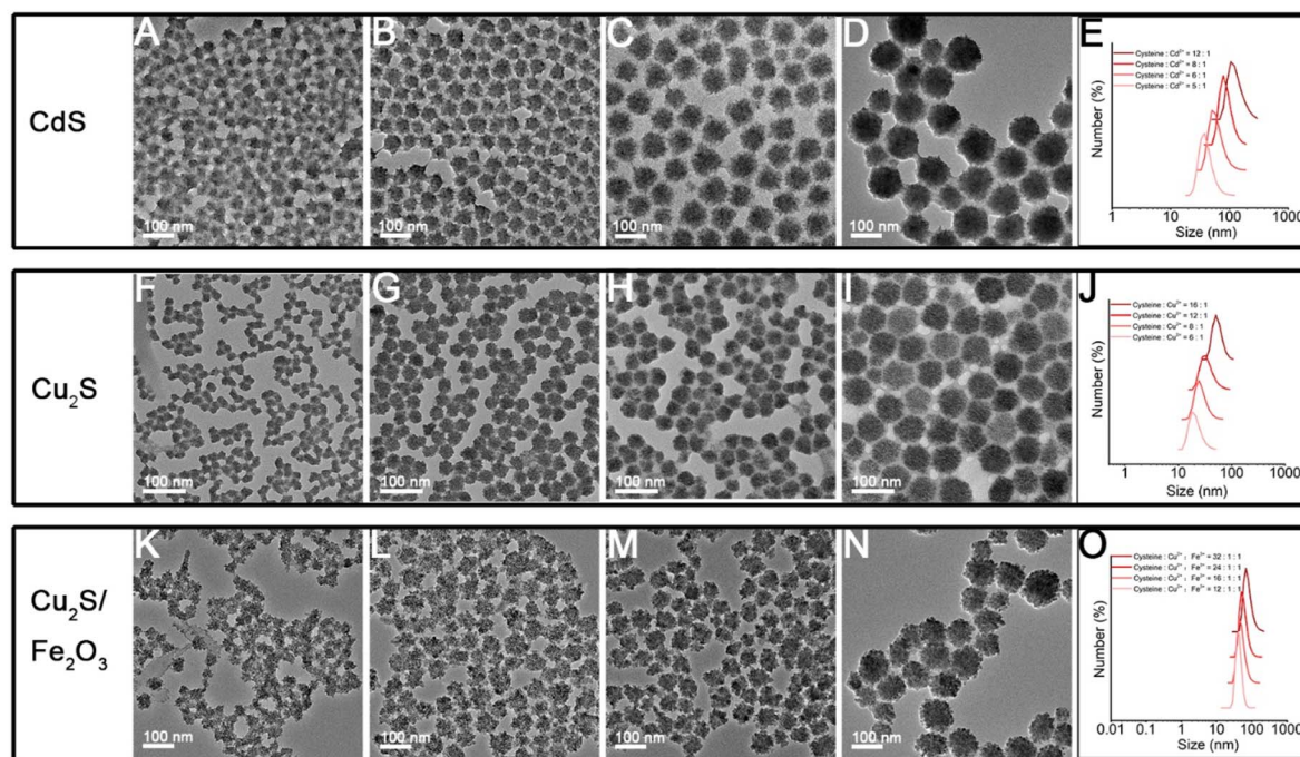
Fig. 6 The size tunability of SPs. (A) TEM image of 33 nm CdS SPs was obtained by adjusting cysteine : \text{Cd}^{2+} = 5 : 1 . (B) TEM image of 44 nm CdS SPs was obtained by adjusting cysteine : \text{Cd}^{2+} = 6 : 1 . (C) TEM image of 75 nm CdS SPs was obtained by adjusting cysteine : \text{Cd}^{2+} = 8 : 1 . (D) TEM image of 104 nm CdS SPs was obtained by adjusting cysteine : \text{Cd}^{2+} = 12 : 1 . (E) Corresponding DLS data of CdS SPs were obtained with different ratios of cysteine to Cd. (F) TEM image of 20 nm \text{Cu}_2\text{S} SPs was obtained by adjusting cysteine : \text{Cu}^{2+} = 6 : 1 . (G) TEM image of 34 nm \text{Cu}_2\text{S} SPs was obtained by adjusting cysteine : \text{Cu}^{2+} = 8 : 1 . (H) TEM image of 39 nm \text{Cu}_2\text{S} SPs was obtained by adjusting cysteine : \text{Cu}^{2+} = 12 : 1 . (I) TEM image of 67 nm \text{Cu}_2\text{S} SPs was obtained by adjusting cysteine : \text{Cu}^{2+} = 16 : 1 . (J) Corresponding DLS data of \text{Cu}_2\text{S} SPs were obtained with different ratios of cysteine to \text{Cu}^{2+} . (K) TEM image of 29 nm \text{Cu}_2\text{S}/\text{Fe}_2\text{O}_3 SPs with different sizes was obtained by adjusting cysteine : \text{Cu}^{2+} : \text{Fe}^{3+} = 12 : 1 : 1 . (L) TEM image of 39 nm \text{Cu}_2\text{S}/\text{Fe}_2\text{O}_3 SPs with different sizes was obtained by adjusting cysteine : \text{Cu}^{2+} : \text{Fe}^{3+} = 16 : 1 : 1 . (M) TEM image of 52 nm \text{Cu}_2\text{S}/\text{Fe}_2\text{O}_3 SPs with different sizes was obtained by adjusting cysteine : \text{Cu}^{2+} : \text{Fe}^{3+} = 24 : 1 : 1 . (N) TEM image of 93 nm \text{Cu}_2\text{S}/\text{Fe}_2\text{O}_3 SPs with different sizes was obtained by adjusting cysteine : \text{Cu}^{2+} : \text{Fe}^{3+} = 32 : 1 : 1 . (O) Corresponding DLS data of \text{Cu}_2\text{S}/\text{Fe}_2\text{O}_3 SPs were obtained with different ratios of cysteine to Cu and Fe.
