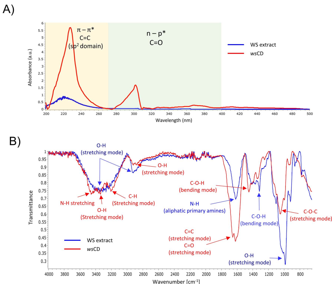
Fig. 2 Chemical structure and surface functional group analysis. (A) Chemical structure analysis of WS extract and ws CDs using UV absorption spectroscopy; (B) surface functional group analysis of WS extract (blue) and ws CDs (red) using Fourier transform infrared spectroscopy.
