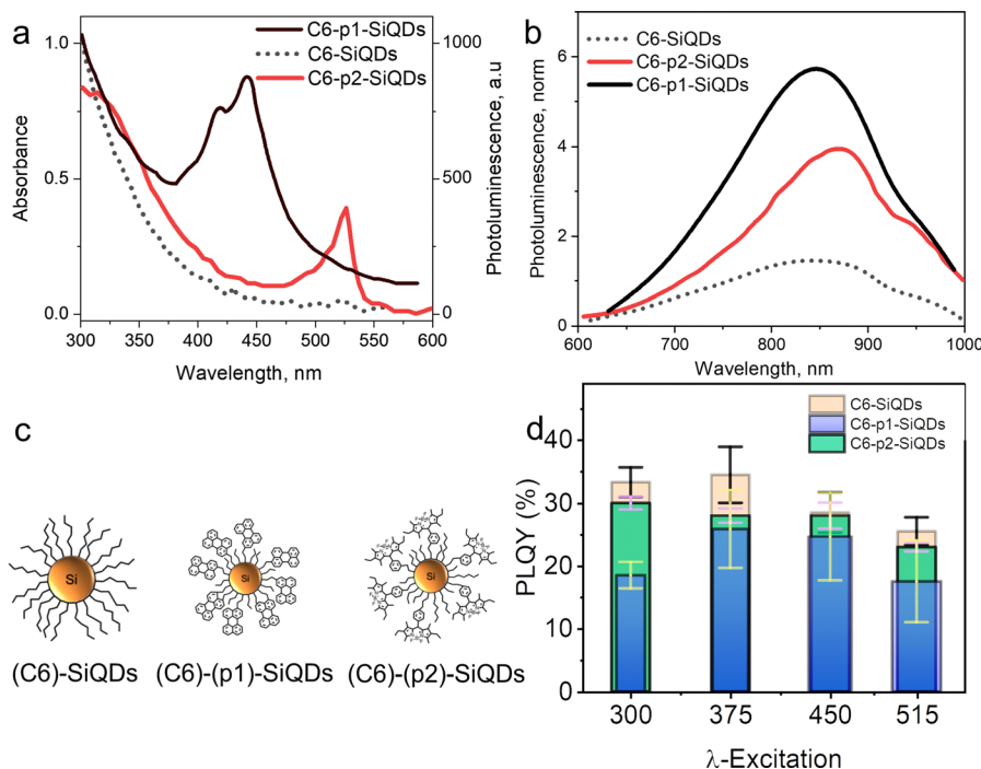
Fig. 11 (a) Absorbance of C6-SiQDs; C6-(p1)-SiQDs; C6-(p2)-SiQDs, (b) PL-emission of C6-SiQDs; C6-(p1)-SiQDs; C6-(p2)-SiQDs, under broadband excitation ( \lambda_{\text{max}} 435–550 nm). (c) Cartoon representation of attributed C6-SiQDs; C6-(p1)-SiQDs; C6-(p2)-SiQDs particles, and (d) PLQY values of C6-SiQDs; C6-(p1)-SiQDs; C6-(p2)-SiQDs measured at different excitation wavelengths. The PLQY values are the result of averaging for five independent synthetic batches. The error bars indicate the maximum and minimum values for five independent synthetic batches. Adapted with permission from ref. 55. Copyright (2020) Royal Society of Chemistry.
