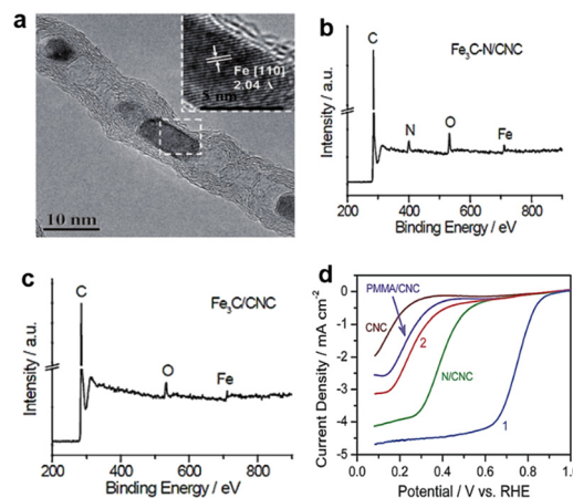
Fig. 4 (a) High resolution transmission electron microscopy (HRTEM) image of \text{Fe}_3\text{C}-\text{N/CNC} with the inset showing the [110] crystal plane of \text{Fe} . 25 XPS spectra of (b) \text{Fe}_3\text{C}-\text{N/CNC} and (c) \text{Fe}_3\text{C/CNC} . 29 (d) ORR performance of \text{Fe}_3\text{C}-\text{N/CNC} (curve 1) and \text{Fe}_3\text{C/CNC} (curve 2). 29
