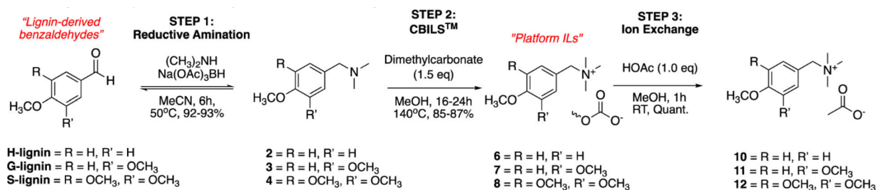
Scheme 20 Three-step synthesis of lignin derived ILs from methylated lignin-derived benzaldehydes. Reproduced with permission from V. Diez, A. DeWeese, R. S. Kalb, D. N. Blanch and A. M. Socha, Ind. Eng. Chem. Res. , 2019, 58 , 16009–16017 (ref. 159). Copyright 2020 American Chemical Society.
