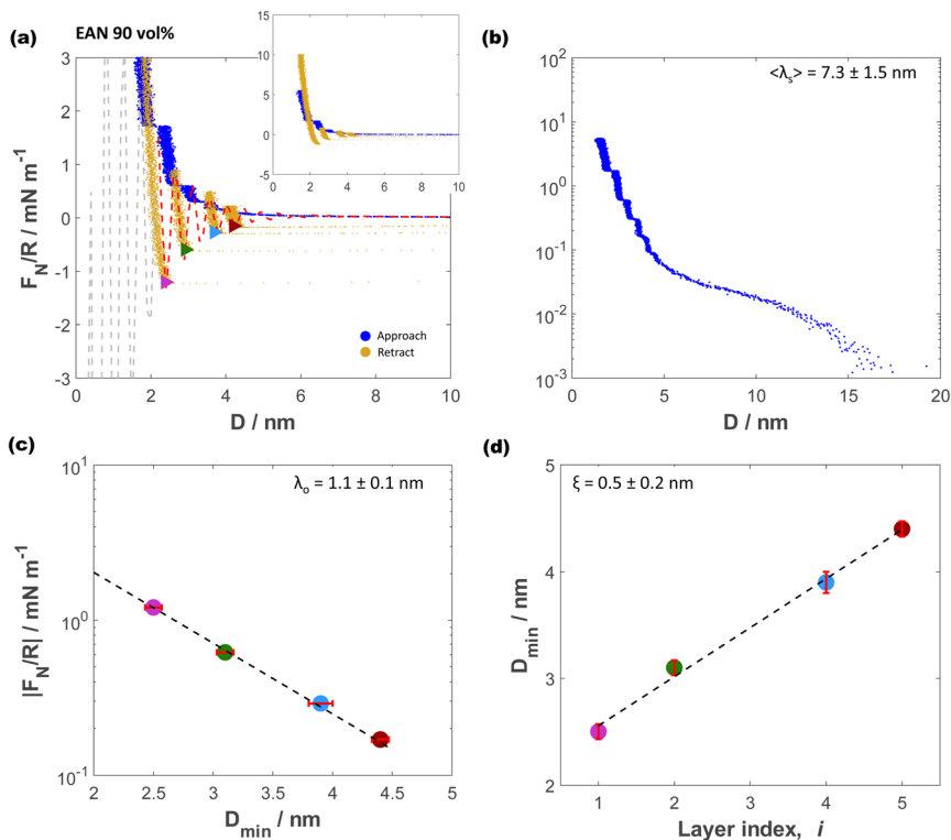
Fig. 3 Example measurements of the normal force between mica sheets as a function of separation, D , across 90 vol% EAN. (a) Linear scale forces at D < 10 nm with retraction (gold) shown from each layer. Red dashed line shows the force fitted using eqn (1) and the parameters reported in Table 1. Inset shows the full magnitude of the force. (b) Log-linear representation of normal force displaying long-range decay with average decay length \langle \lambda_s \rangle = 7.3 \pm 1.5 nm. (c) The exponential decay envelope is calculated from the force minima, giving \lambda_o = 1.1 \pm 0.1 nm. (d) The distance separation between the minima gives the oscillation wavelength of the structural force, here \xi = 0.5 \pm 0.2 nm.
