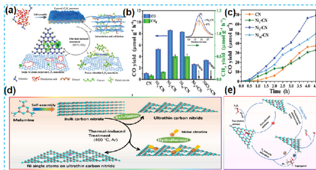
Fig. 17 (a) Schematic illustration for the synthesis of \text{Ni}_5\text{-CN} . (b) Photocatalytic products of \text{CO}_2 reduction over \text{Ni}_5\text{-CN} under visible light illumination for 1 h, in comparison with CN, \text{Ni}_1\text{-CN} , \text{Ni}_{10}\text{-CN} , and CN with nickel powders, and CN with \text{NiCl}_2 . (c) The reaction proceeds upon illumination for 4.5 h. 75 (d) Schematic illumination for the fabrication of the NiCN-4 catalyst. (e) Schematic demonstration of photocatalytic \text{H}_2\text{O}_2 generation for the NiCN-4 catalyst under visible light irradiation. 77
