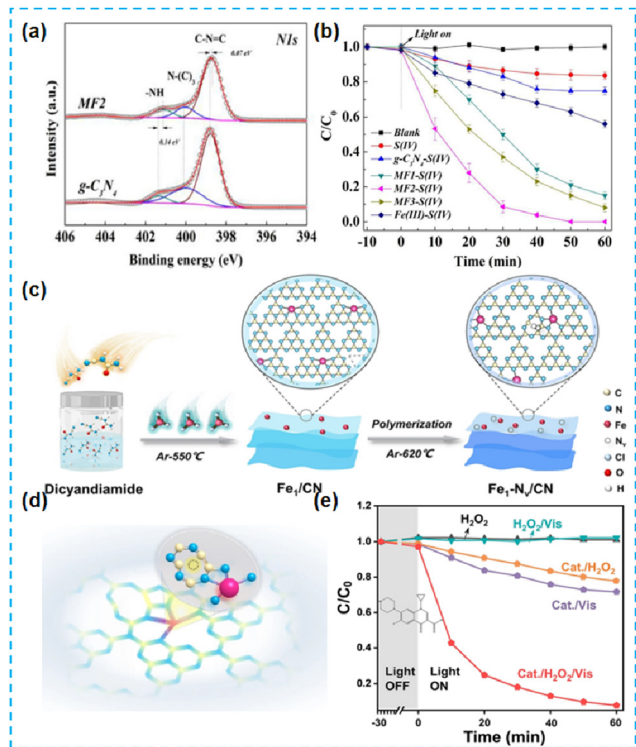
Fig. 15 (a) High resolution XPS spectra of g\text{-C}_3\text{N}_4 images of MF2 (Fe deposited g\text{-C}_3\text{N}_4 ). (b) DCF degradation by different systems. 70 (c) Synthesis of \text{Fe}_1\text{-N}_x/\text{CN} ultrathin nanosheets. (d) Schematic model of \text{Fe}_1\text{-N}_x/\text{CN} . (e) Degradation curves of CIP in a solely photocatalytic process, Fenton reaction, and photocatalytic activation \text{H}_2\text{O}_2 process with or without \text{Fe}_1\text{-N}_x/\text{CN} . 71
