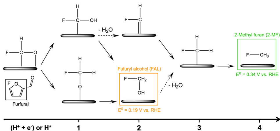
Scheme 1 Proposed reaction mechanisms for the furfural electroreduction reaction towards furfuryl alcohol (FAL) and 2-methylfuran (2-MF) on Cu surfaces. 17,18 (H + + e - ) and H* denote proton-coupled electron transfer (PCET) and surface hydrogenation (where H* is produced via the Volmer reaction), respectively. The solid or dashed arrows represent elementary reduction step without or with H 2 O production.
