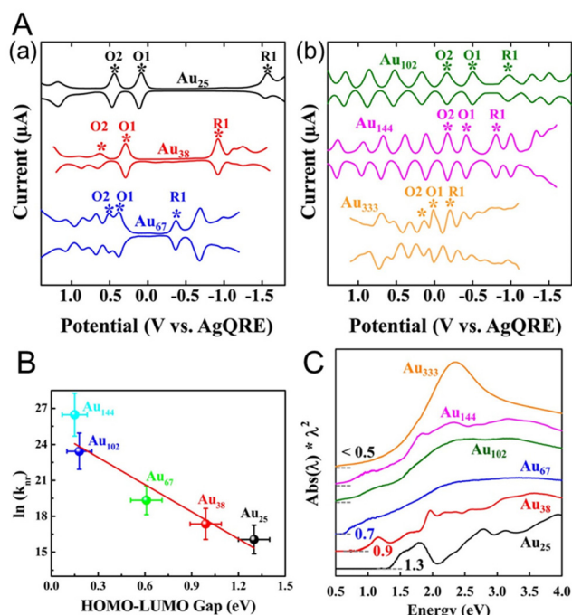
Fig. 5 (A) Square-wave voltammograms of (a) \text{Au}_{25}(\text{SC}_6\text{H}_{13})_{18} , \text{Au}_{38}(\text{SC}_6\text{H}_{13})_{24} , and \text{Au}_{67}(\text{SC}_6\text{H}_{13})_{35} and (b) \text{Au}_{102}(\text{SC}_6\text{H}_{13})_{44} , \text{Au}_{144}(\text{SC}_6\text{H}_{13})_{60} , and \text{Au}_{333}(\text{SC}_6\text{H}_{13})_{79} in \text{CH}_2\text{Cl}_2 containing 0.1 M TBAPF 6 . (B) Plot of \ln(k_{\text{nr}}) versus the H–L gap for gold clusters. The solid line is the best fit straight line for the data ( \text{Au}_{25} – \text{Au}_{144} ). (C) Ultraviolet–visible–near-infrared absorption spectra of \text{Au}_{25}(\text{SC}_6\text{H}_{13})_{18} , \text{Au}_{38}(\text{SC}_6\text{H}_{13})_{24} , \text{Au}_{67}(\text{SC}_6\text{H}_{13})_{35} , \text{Au}_{102}(\text{SC}_6\text{H}_{13})_{44} , \text{Au}_{144}(\text{SC}_6\text{H}_{13})_{60} , and \text{Au}_{333}(\text{SC}_6\text{H}_{13})_{79} . Reproduced with permission from ref. 88. Copyright 2017, American Chemical Society.
