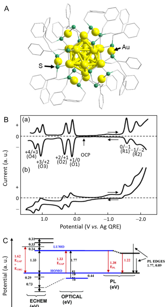
Fig. 4 (A) Geometric structure of [\text{Au}_{25}(\text{PET})_{18}]^- . (B) (a) 25 °C DPVs at 0.02 V \text{s}^{-1} , and (b) -70 °C cyclic voltammogram (0.1 V \text{s}^{-1} ) of \text{Au}_{25}(\text{PET})_{18} in 0.1 M TBAPF 6 in degassed \text{CH}_2\text{Cl}_2 with a 0.4 mm-diameter Pt WE, a Ag-wire quasi-RE, and a Pt-wire CE. The arrows indicate the solution rest potentials, and * indicates the wave for incompletely removed \text{O}_2 , which varied from experiment to experiment. (C) Energy level diagram for \text{Au}_{25}(\text{PET})_{18} based on the data in \text{CH}_2\text{Cl}_2 solution. Reproduced with permission from ref. 74. Copyright 2004, American Chemical Society.
