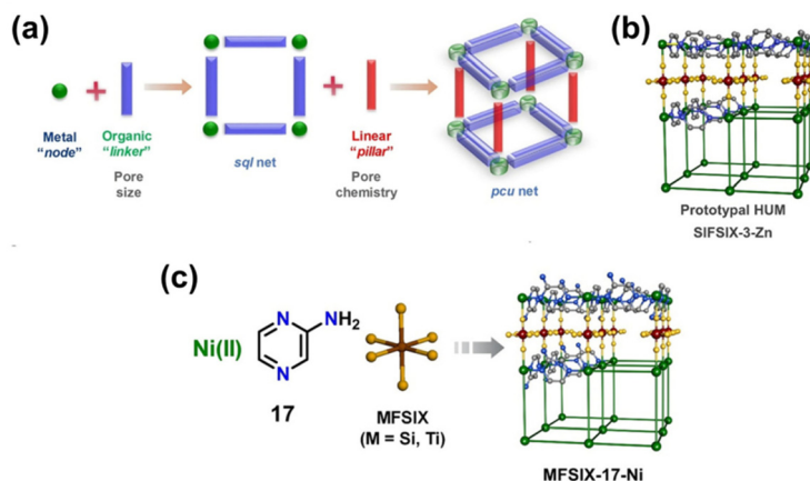
Fig. 2 (a) Schematic illustration of the modularity of pillared square grids that form the pcu topology of HUMs, (b) the prototypical pyrazine (pyz) linked HUM [\text{Zn}(\text{pyz})_2(\text{SiF}_6)]_n , and (c) schematic illustration of the building blocks. 64 Reproduced with permission, Copyright 2021 John Wiley & Sons, Inc.
