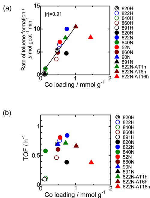
Fig. 10 (a) Toluene formation rate at 3 h of time on stream plotted as a function of Co loading for Co/MFI catalysts. The Co/MFI catalysts were prepared using a \text{Co}(\text{OAc})_2 solution ( 200 \text{ mmol L}^{-1} ) at 343 K for 4 h. The linear plot was made without the addition of the data of 822N-AT16h. (b) TOF ( \text{h}^{-1} ) plotted as a function of Co loading. The TOF values were calculated based on the toluene formation rate at 3 h of time on stream from the beginning of the reaction and the Co loading.
