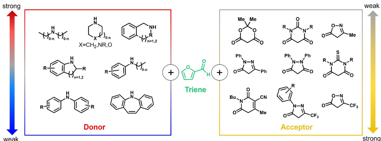
Fig. 2 DASA synthesis and building blocks. (a) DASA synthesis is modular and based on the Knoevenagel condensation of furfural with a cyclic \beta -keto carbonic acid, followed by a ring-opening reaction of the resulting furan adduct with a secondary amine. (b) Chemical structures of different secondary amine donors and carbon acid acceptors previously utilized for DASA synthesis. Donors and acceptors are ranked tentatively according to their approximate strength (as indicated by reported or predicted pK_a(H) ). The properties of DASAs are largely dictated by the relative strength of their donor and acceptor groups. The triene bridge of the open isomer is derived from furfural.
