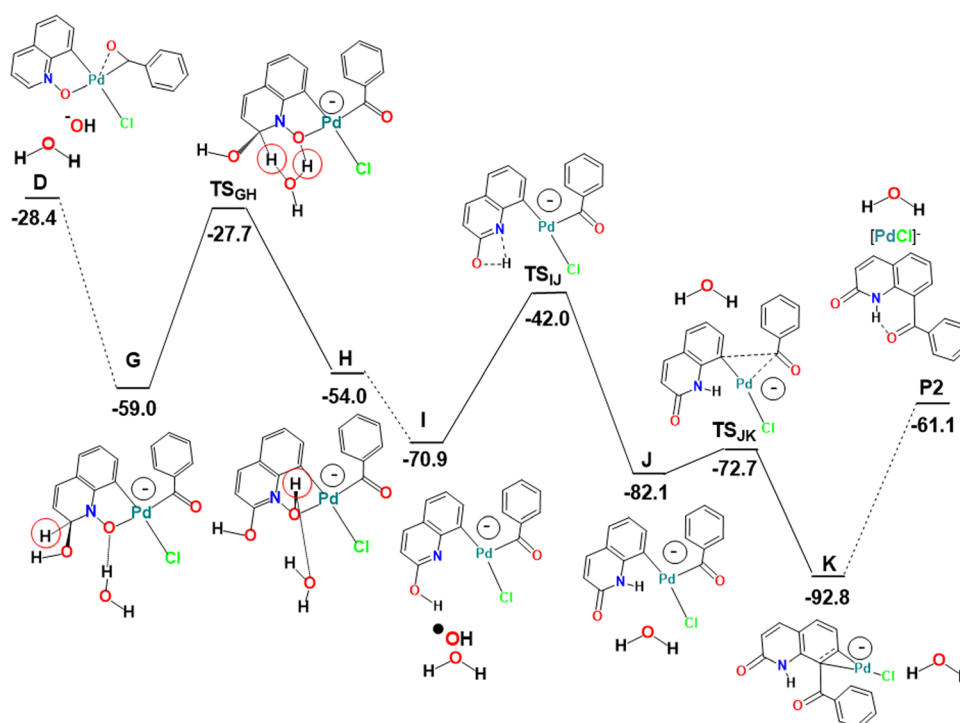
Fig. 3 Energy profile for the second part of the alternative functionalization at C8 and functionalization at C2 of QO in the presence of water (relative Gibbs energies in \text{kcal mol}^{-1} in dichloroethane; the negative charge represents the charge of the complex and the red circle highlights the hydrogen migrating in the G to H transformation).
