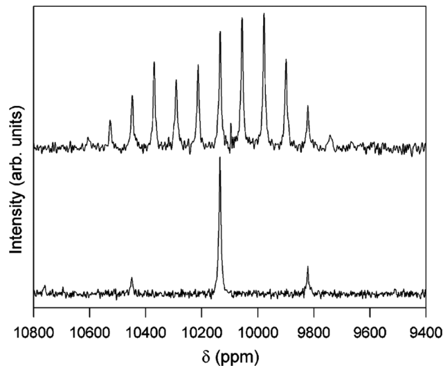
Fig. 12 ^1\text{H} - ^{103}\text{Rh} CP-MAS NMR spectra of [(\text{H}_2\text{O})_4\text{Rh}(\mu_2\text{-OH})_2\text{Rh}(\text{H}_2\text{O})_4(\text{dmto})_4] \cdot 8\text{H}_2\text{O} comparing spinning rates of 1.0 (top) and 4.0 kHz (bottom). Both spectra acquired with 8 ms contact time, 5 s relaxation delay for 12 000 (top) and 15 800 (bottom) acquisitions. 37 Reproduced from the ref. 37 with permission from the American Chemical Society, copyright 2006.
