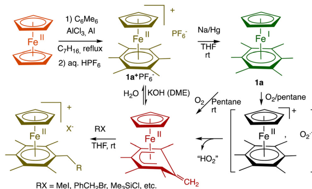
Scheme 1 Synthesis and reaction with O_2 of the 19-electron Fe(I) complex 1a . Due to the large difference (about 1 V) between the two redox systems Fe(I)/Fe(II) and O_2/O_2^{\bullet-} , electron transfer from Fe(I) to O_2 is very exergonic and fast, followed by deprotonation by O_2^{\bullet-} within the intermediate ion cage (from O_2^{\bullet-} EPR). 14,15 In THF, this cage superoxide reaction is totally inhibited by NaPF 6 due to ion exchange between the two ion pairs [Fe(II) + , O_2^{\bullet-} ] and [Na + , PF 6 - ], 16 (for a review of salt effects, see ref. 17) which is reminiscent of the function of superoxide dismutase enzyme. 18
