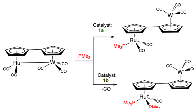
Scheme 2 ETC-catalyzed \text{PMe}_3 ligand addition in the fulvalene heterobimetallic complex [\text{RuW}(\eta^{10}\text{-}\mu^2\text{-C}_{10}\text{H}_8)(\text{CO})_5] . The reaction depends on the \text{Fe(II/I)} redox potential of the electron-reservoir ETC catalyst ( 1a vs. [\text{Fe}(\eta^5\text{-C}_5\text{Me}_5)(\eta^6\text{-C}_6\text{Me}_6)] , 1b ). With the more electron-rich electron reservoir 1b as ETC catalyst, two \text{PMe}_3 ligands are introduced whereas, with 1a , only one \text{PMe}_3 ligand is added. ETC catalysis was pioneered by Henry Taube. 27
