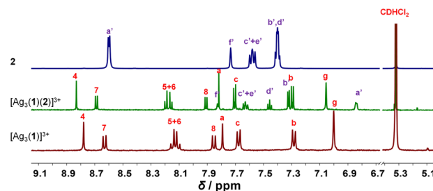
Fig. 1 Partial ^1\text{H} NMR (600 MHz, \text{CD}_2\text{Cl}_2 , 298 K) of silver(i)-loaded deck [\text{Ag}_3(\mathbf{1})(\mathbf{2})]^{\mathbf{3}+} , slider-on-deck [\text{Ag}_3(\mathbf{1})(\mathbf{2})]^{\mathbf{3}+} and biped 2 .
