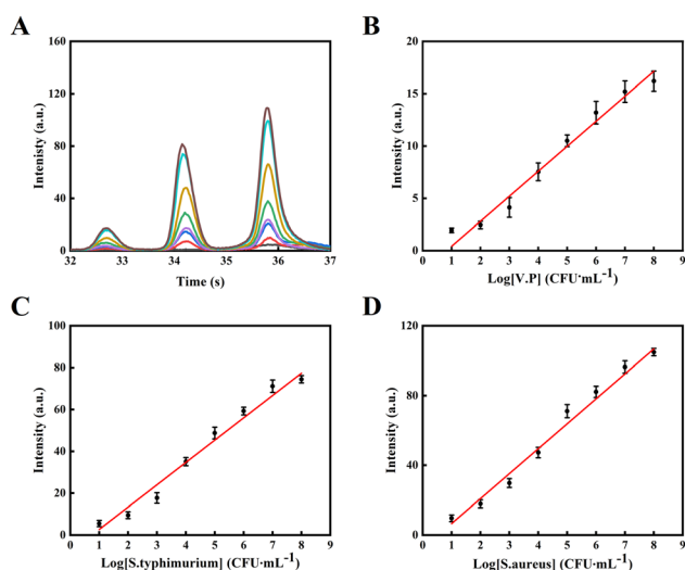
Fig. 6 (A) Microfluidic chip technology determination of V.P, S.T, and S. A in the concentration range from 10 CFU mL ^{-1} to 1 \times 10^8 CFU mL ^{-1} . (B), (C), and (D) Correspond to the calibration plots for V.P, S.T, and S.A, respectively. (The signal probe was 0.2 \mu M and the capture probes were 0.02 \mu M, pH was 8.0, the reaction buffer was PBS buffer, and time was 0.5 h).
