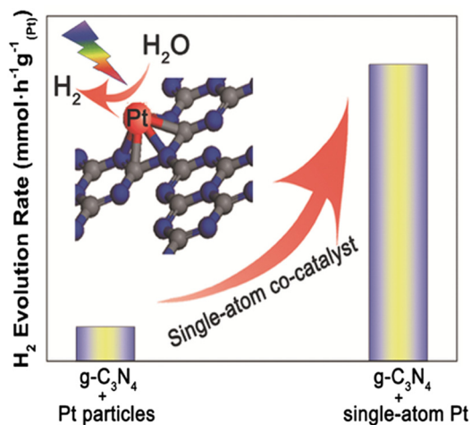
Fig. 24 The highly stable single-atom co-catalyst (Pt) embedded in the sub-nanoporosity of 2D g-C 3 N 4 leading to significantly enhanced photo-catalytic H 2 evolution activity. Reprinted with permission from John Wiley and Sons. 286
