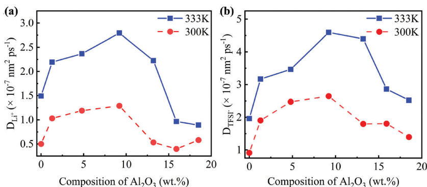
Fig. 3 Diffusivities of (a) \text{Li}^+ and (b) TFSI ^- at different temperatures in the SC system.
