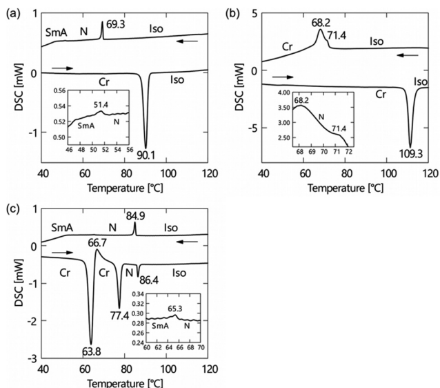
Fig. 2 DSC curves of (a) (\pm) -1, (b) (\pm) -2 and (c) (\pm) -3. A standard notation gives the transition temperatures between the crystalline (Cr), smectic A (SmA), nematic (N) and isotropic (Iso) phases.
