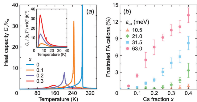
Fig. 8 (a) Temperature dependence of the heat capacity for different values of x . The inset shows C_v/T^3 vs. T curves. Simulation parameters: \epsilon_1 = 21 meV, \epsilon_2 = 12.6 meV, \epsilon_{\text{Cs}} = 31.5 meV, L = 10 . (b) Fraction of the frustrated FA cations in the ordered phase vs. x for different \epsilon_{\text{Cs}} interaction energies. Simulation parameters: \epsilon_1 = 21 meV, \epsilon_2 = 12.6 meV, L = 10 ; data averaged over 10 independent simulation runs.
