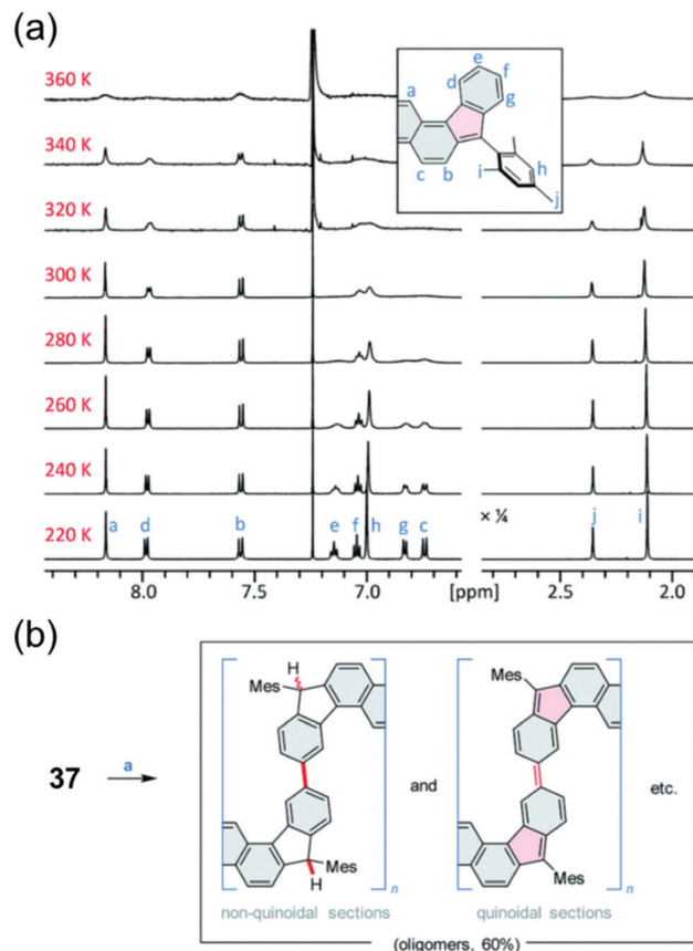
Fig. 19 (a) Temperature-dependent ^1\text{H} NMR spectra of 37 ( \text{CDCl}_3 , 600 MHz). The signals were assigned at 220 K using 2D spectroscopic methods (see ref. 234 for details). (b) Thermally induced oligomerization of 37. Reagents and conditions: (a) argon, pressure tube, 240 °C, 14 h. Reproduced from ref. 234 under CC BY-NC 3.0 licence.
