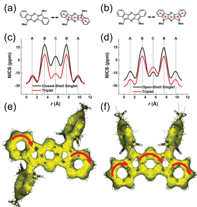
Fig. 16 Comparison of the resonance structures of (a) 25 and (b) 30 . NICS-XY scans of (c) 25 and (d) 30 . ACID plots of (e) closed-shell singlet 25 and (f) open-shell triplet 30 at an isosurface (yellow) value of 0.04. The general aromatic current is indicated by the superimposed clockwise red arrows. Reproduced with permission from ref. 11 Copyright 2020 Wiley-VCH GmbH.
