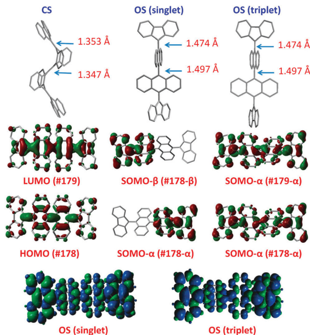
Fig. 18 Calculated geometric structures (with part of the bonds labelled with length in Å) and the frontier molecular orbitals of the closed-shell (CS) and open-shell (OS) forms of 36 both in singlet and in triplet states. The bottom panel shows the spin density distributions of the singlet and triplet open-shell forms of 36 . Reprinted (adapted) with permission from ref. 224 Copyright 2012 American Chemical Society.
