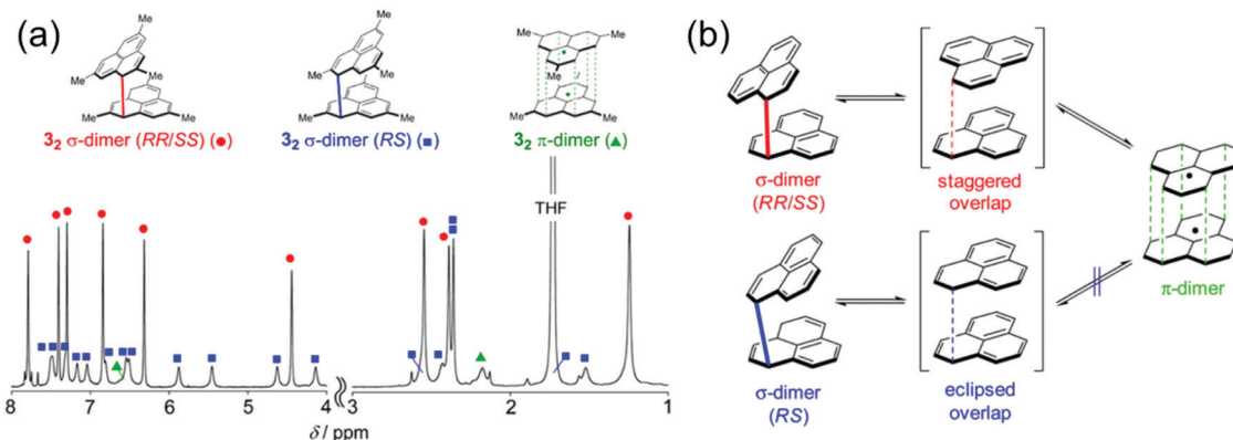
Fig. 13 (a) ^1\text{H} NMR spectrum of methyl-substituted phenalenyl dimers measured in degassed \text{THF-d}_8 at 173 K. The aromatic and olefinic region (8–4 ppm) is magnified 3 times relative to the aliphatic region (3–1 ppm) for ease of visualization. (b) Dynamic Exchange between the dimers (methyl groups are omitted for clarity). Reprinted (adapted) with permission from ref. 162 Copyright 2016 American Chemical Society.
