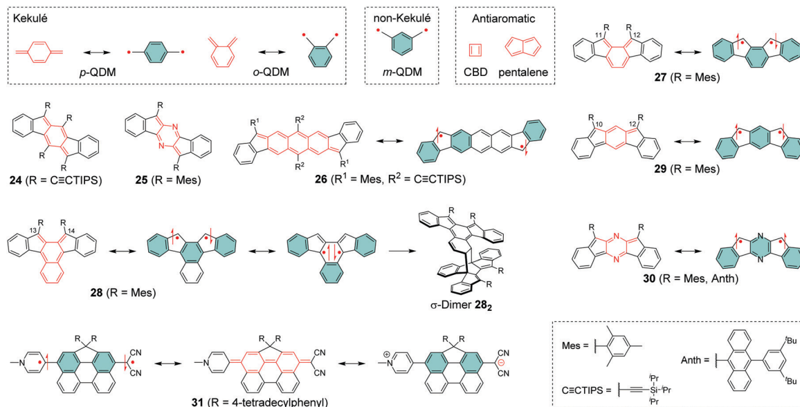
Scheme 8 Delocalised diradicals and their closed-shell and open-shell resonance structures (R groups are omitted from some resonance structures for clarity).
