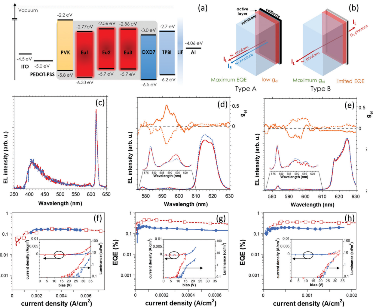
Fig. 2 (a) Flat-band energy level diagram of the CP-OLEDs, (b) Structure of type A (reflective cathode) and type B (transparent cathode) devices; CP-EL spectra (solid red and dashed blue lines for the two CP components) of devices embedding Eu1 (c), Eu2 (d) and Eu3 (e) with transparent cathode (inset: expansion of the EL between 575 and 610 nm), and g_{\text{el}} (orange lines, continuous for (S,S), dashed for (R,R) enantiomer) for Eu2–3 ; corresponding EQE vs. J of type A (red \square ) and B devices (blue \bullet ) embedding Eu1 (f), Eu2 (g) and Eu3 (h); in the insets, corresponding current density–voltage curves (solid lines) and Luminance–voltage (dashed lines) of type A (red \square ) and B devices (blue \bullet ).
