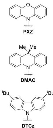
Fig. 1 BP-based TADF emitters; DMAC: 9,9-dimethyl-9,10-dihydroacridine, PXZ: 10H-phenoxazine, DTCz: 3,6-di-tert-butylcarbazole.
