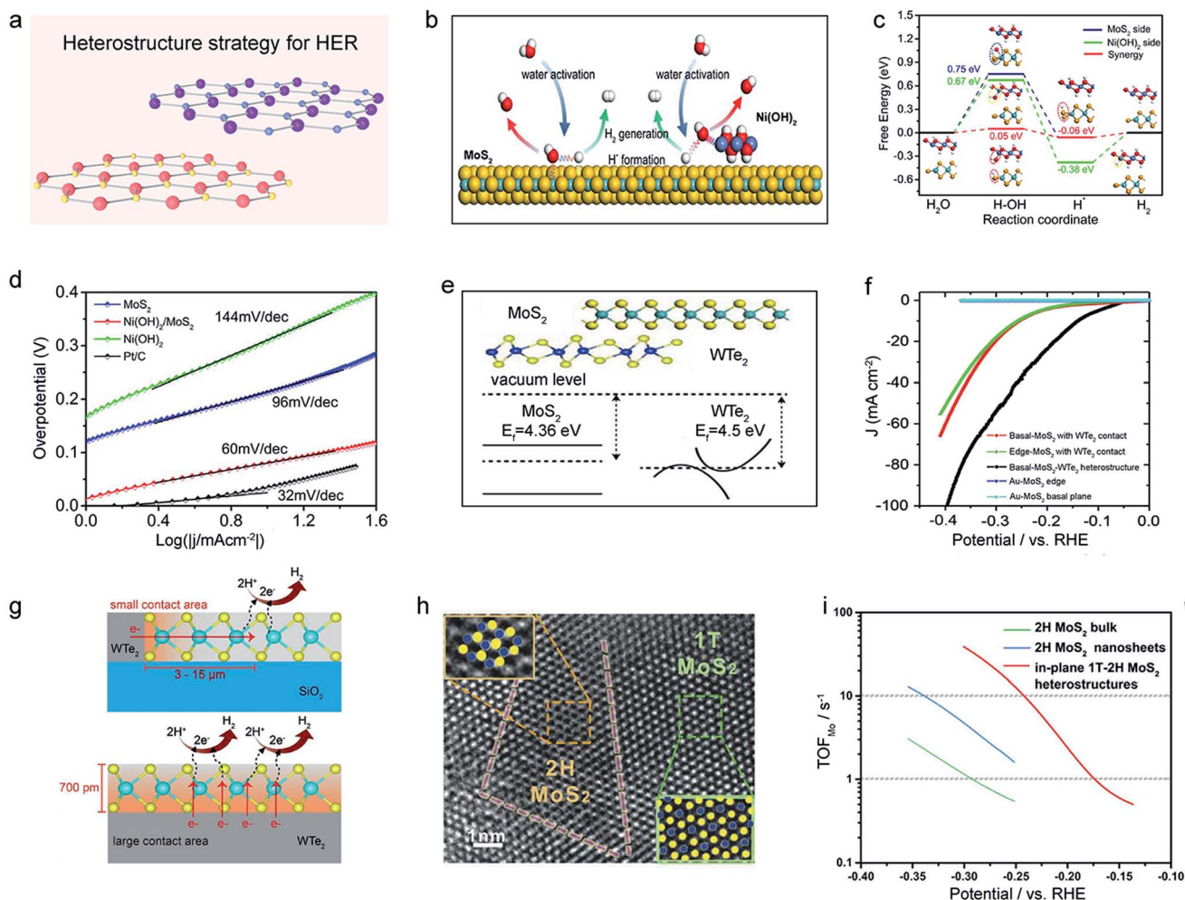
Fig. 13 Heterostructure strategy of 2D-TMDCs for HER. (a) Schematic illustration of the heterostructure strategy for HER. (b) Schematic illustration of the water activation process for the \text{Ni}(\text{OH})_2/\text{MoS}_2 heterostructure in an alkaline solution. H, O, Mo, S, and Ni atoms are shown in white, red, cyan, yellow, and blue, respectively. The free energy diagram (c) and the Tafel plots (d) for \text{MoS}_2 , \text{Ni}(\text{OH})_2 , and \text{Ni}(\text{OH})_2/\text{MoS}_2 . Reproduced with permission, 188 Elsevier. (e) The aligned band structure of the \text{MoS}_2/\text{WTe}_2 heterostructure. (f) The corresponding polarization curves of the \text{MoS}_2/\text{WTe}_2 heterostructure. (g) Comparison of the HER mechanisms of the \text{MoS}_2/\text{WTe}_2 heterostructure (bottom) and \text{MoS}_2 with \text{WTe}_2 edge-contact (top). Reproduced with permission, 189 Wiley-VCH. HRTEM image (h) and the TOF (i) of the in-plane 1T-2H \text{MoS}_2 heterostructure. Reproduced with permission, 125 Wiley-VCH.
