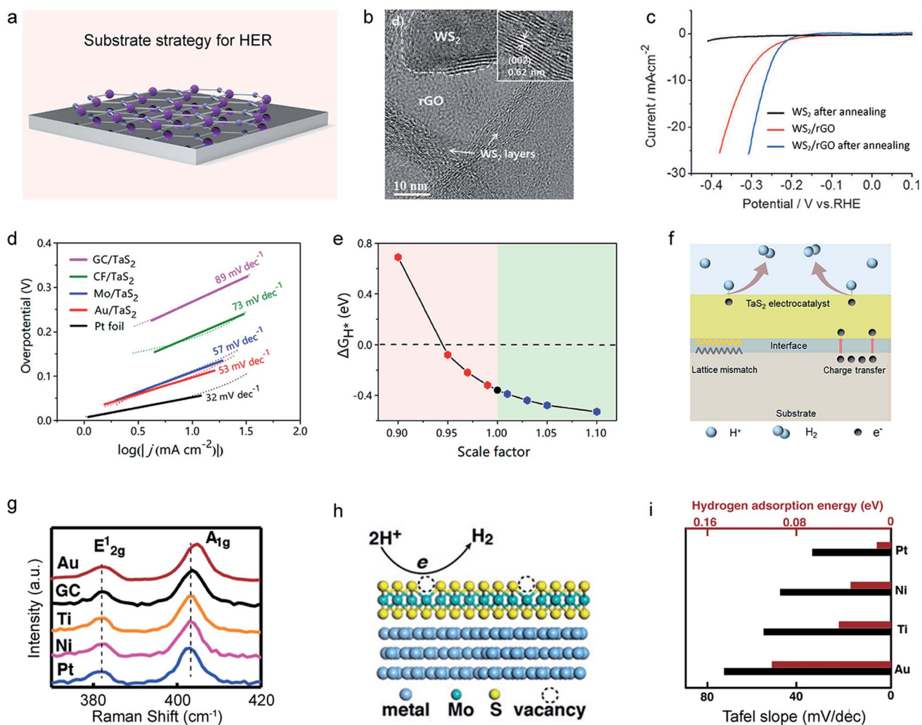
Fig. 12 Substrate strategy of 2D-TMDCs for HER. (a) Schematic illustration of the substrate strategy for HER. (b) HRTEM image of the WS_2 /reduced graphene oxide ( WS_2 /rGO) hybrid nanosheet. Inset: the zoom-in image of the WS_2 nanosheet. (c) Polarization curves of the annealed WS_2 /rGO hybrid nanosheets, in comparison to those of annealed WS_2 nanosheets and WS_2 /rGO hybrid nanosheets. Reproduced with permission, 155 Wiley-VCH. (d) Tafel plots of TaS_2 samples on glass carbon (GC), carbon fibers (CF), Mo, and Au substrates. (e) The \Delta G_{H^+} of the TaS_2 nanosheet under the lattice-mismatch condition. (f) Schematic illustration of the substrate effect on a TaS_2 electrocatalyst. Reproduced with permission, 156 American Chemical Society. (g) Raman spectra of monolayer MoS_2 on Au, GC, Ti, Ni, and Pt substrates, showing the redshift of Pt > Ni > Ti > Au. (h) Schematic illustration of the substrate effect on a MoS_2 monolayer. (i) Calculated hydrogen adsorption energies and the measured Tafel slopes of a MoS_2 monolayer on Pt, Ni, Ti, and Au substrates. Reproduced with permission, 40 American Chemical Society.
