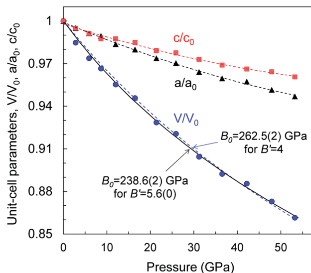
Fig. 4 Pressure dependencies of relative variations in the unit-cell volume and lattice parameters of a WB_4 single crystal at 295 K. Error bars are smaller than symbols' size.
