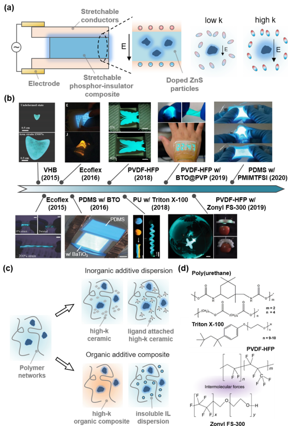
Fig. 16 High- k SIs for low-voltage optoelectronics. (a) Structure of stretchable alternate-current-electroluminescence (ACCEL) devices. The phosphors exhibit higher luminescence under an electric field, when the surrounding medium has higher dielectric constants. (b) Materials development for low voltage stretchable ACCEL devices. Reproduced with permission from ref. 155, 156, 157, 158 and 159. Copyright 2015, 2016, 2018, and 2020, Wiley-VCH. Reproduced with permission from ref. 26. Copyright 2016, AAAS. Reproduced with permission from ref. 160 and 161. Copyright 2018, and 2019, The American Chemical Society. (c) Schematics of strategies used to develop high- k stretchable dielectrics. (d) Molecular structures comprising high- k organic composites. Reproduced with permission from ref. 162. Copyright 2019, Springer Nature.
