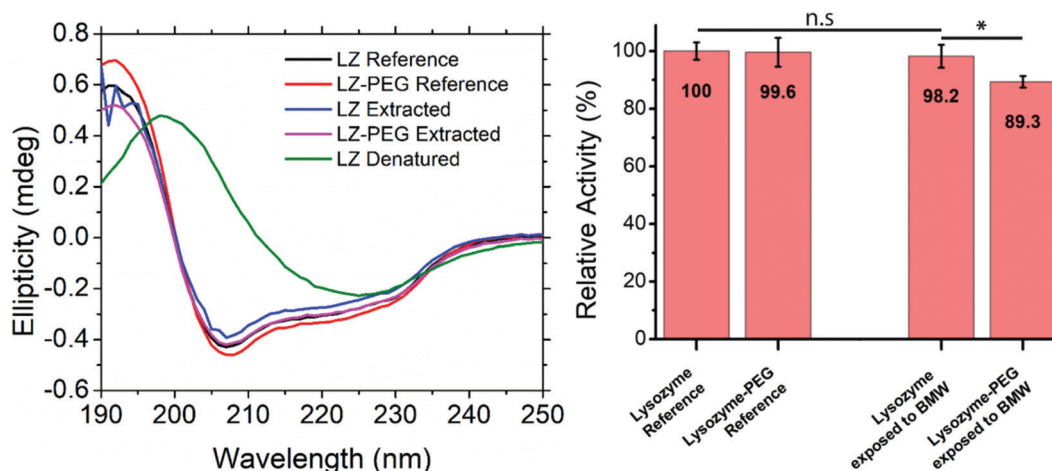
Fig. 4 (A) CD spectra of a LZ and PEG-LZ reference compared to LZ and PEG-LZ extracted from a BMW mixture and a solution of denatured LZ. (B) Relative enzymatic activity of LZ and PEG-LZ in 1 \times PBS buffer compared to LZ and PEG-LZ exposed to the BMW solvent mixture, dried and resolubilised in 1 \times PBS buffer. The concentration of all samples was 5000 ng mL -1 , and each condition was duplicated into 4 wells, measured and averaged. The error bars represent the standard deviation. * is determined using a two-sample t -test, and represents statistical significance at 0.01 < p < 0.05.
