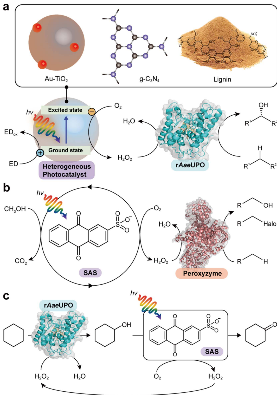
Fig. 6 Photocatalytic formation of H 2 O 2 and selective oxidation reactions catalyzed by rAaeUPO and peroxozyme. Representative photocatalysts include Au-TiO 2 , 90 g-C 3 N 4 , 95 lignin 99 (a), and anthraquinone (SAS) 97,106 (b). (c) Photocatalytic oxidation of cyclohexane to cyclohexanone. The SAS-catalyzed aerobic overoxidation of cyclohexanol to cyclohexanone produces H 2 O 2 as a byproduct, which itself is used to support the rAaeUPO-catalyzed hydroxylation of cyclohexane. 97
