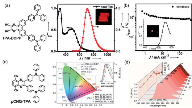
Fig. 2 (a) The absorption (black) and PL (red) spectra of TPA-DCPP in a neat film. Inset: image of the neat film under UV irradiation ( \lambda_{\text{ex}} = 365 nm). Copyright 2015, John Wiley & Sons. (b) EQE versus current density characteristics of the TPA-DCPP based non-doped device. Inset: EL spectrum and image of the device at 5 V. Copyright 2015, John Wiley & Sons. (c) Coordinates of the devices in CIE space and corresponding EL spectra (insets). Copyright 2021, John Wiley & Sons. (d) Variations of photoluminescence (PL) spectra and PL quantum yields for CBP: x % p CNQ-TPA films ( x = 10–100). Copyright 2021, John Wiley & Sons.
