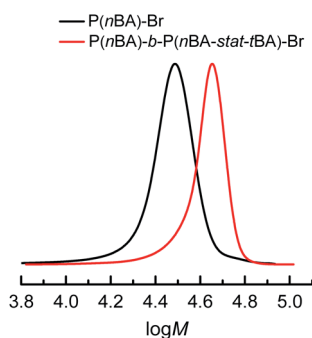
Fig. 5 Molecular weight distribution of P(nBA)_{288}-Br macroinitiator ( M_n = 37.0 kDa and D = 1.11 , conv_{BA} = 83\% ) and P(nBA)_{288}-b-P(nBA)_{40}-stat-tBA_{56}-Br copolymer ( M_n = 50.6 kDa and D = 1.06 , conv_{tBA} = 25\% , conv_{BA} = 94\% ) produced by PGE eATRP of nBA and nBA + tBA at T = 45^\circ C in DMF + 0.1 M Et_4NBF_4 . tBA was added after 1 h of nBA polymerization under the following conditions: nBA/EBiB/Cu(OTf)_2/Me_6TREN/Et_4NBr = 349/1/0.1/0.3/0.1 , C_{nBA} = 3.49 M.
