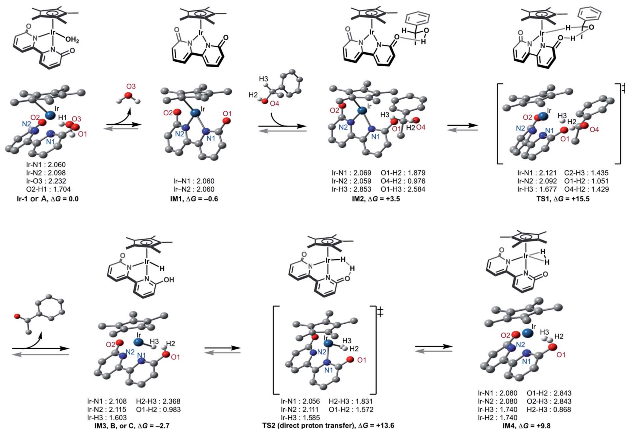
Fig. 5 Geometry and energy changes of the proposed pathway at the CAM-B3LYP + GD3 level of theory using SDD and 6-31++G** basis sets for Ir and other atoms, respectively. Solvent effect (H 2 O) by IEFPCM method; Gibbs free energies in kcal mol -1 at T = 353.15 K.
