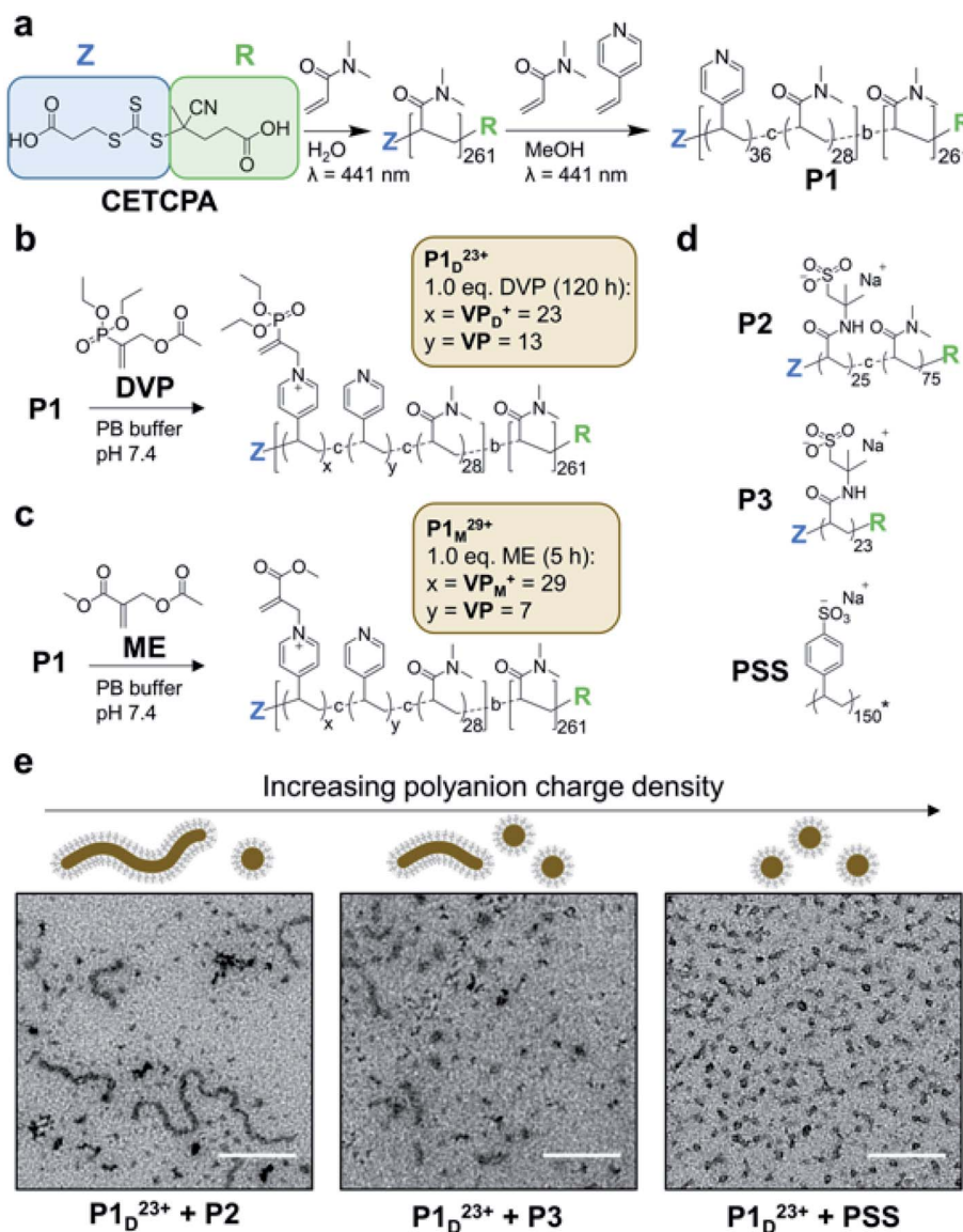
Fig. 2 Polyamine block copolymer (P1) synthesis and assembly into C3Ms. (a) Two step synthesis of P1 from RAFT polymerisation of DMA and 4VP with chain transfer agent (4-((((2-carboxyethyl)thio)carbonothioyl)thio)-4-cyanopentanoic acid, CETCPA). (b) Conversion of neutral VP units to cationic VP_{D^+} in P1 (20 mM) by reaction with DVP (1.0 eq.) in pH 7.4 PB buffer (100 mM) yielding P1_{D^{23+}} . (c) Conversion of neutral VP to cationic VP_{M^+} in P1 (20 mM) by reaction with ME (1.0 eq.) in pH 7.4 PB buffer (100 mM) yielding P1_{M^{29+}} . Acetate counterions in P1_{D^{23+}} and P1_{M^{29+}} omitted for visual clarity. (d) Structures of polyanions combined P1_{D^{23+}} during initial micelle assembly studies. P2 and P3 were synthesised by RAFT polymerisation of 2-acrylamido-2-methylpropane sulfonic acid (AMPS) and DMA with CETCPA as the chain transfer agent. Poly(sodium 4-styrenesulfonate) (PSS) was commercially obtained with a reported MW of 200 kDa, while M_{n, GPC} = 31.5 kDa was measured in our laboratory. *The average degree of polymerisation (150) as shown in the figure is therefore a conservative estimate based on M_{n, GPC} to highlight its relatively high charge density. (e) TEM images and schematic illustration of coacervate core micelles (C3Ms) obtained from the combination of P1_{D^{23+}} with polyanions of varied charge density at 4 mM amine and anionic functional group concentration (scale bar is 200 nm). Samples were visualised with uranyl acetate staining. Additional TEM, cryoTEM and DLS data are presented in Fig. S11–S12.†
