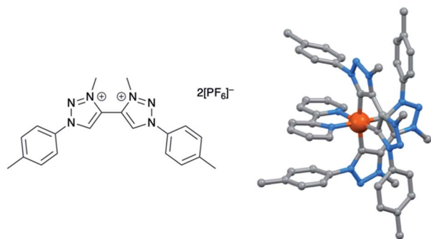
Fig. 13 The 1,2,3-triazol-5-ylidene-containing compound [H 2 btz][PF 6 ] 2 and the structure of [Fe(bpy)(btz)] 2+ (CSD refcode NOVAX).
